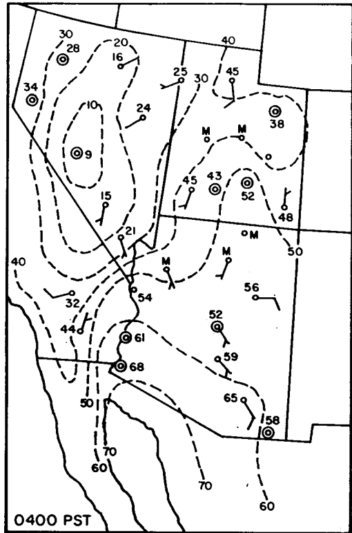
FIG. 4. Surface isodrosotherm analysis for 0400 LST 3 July 1975.
