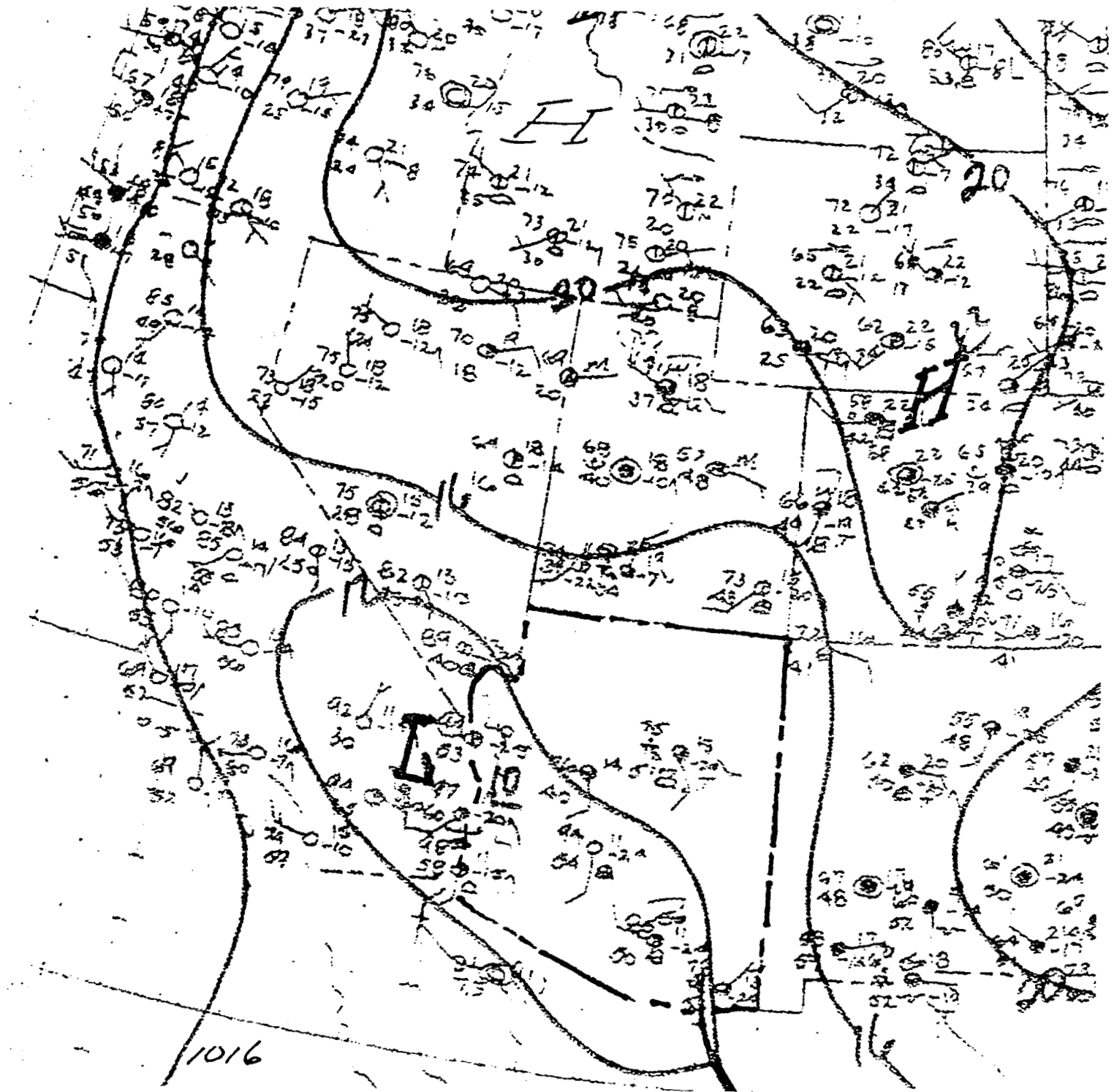
FIGURE 9--SURFACE MAP FOR 2:00 P.M., SEPTEMBER 14, 1974.
