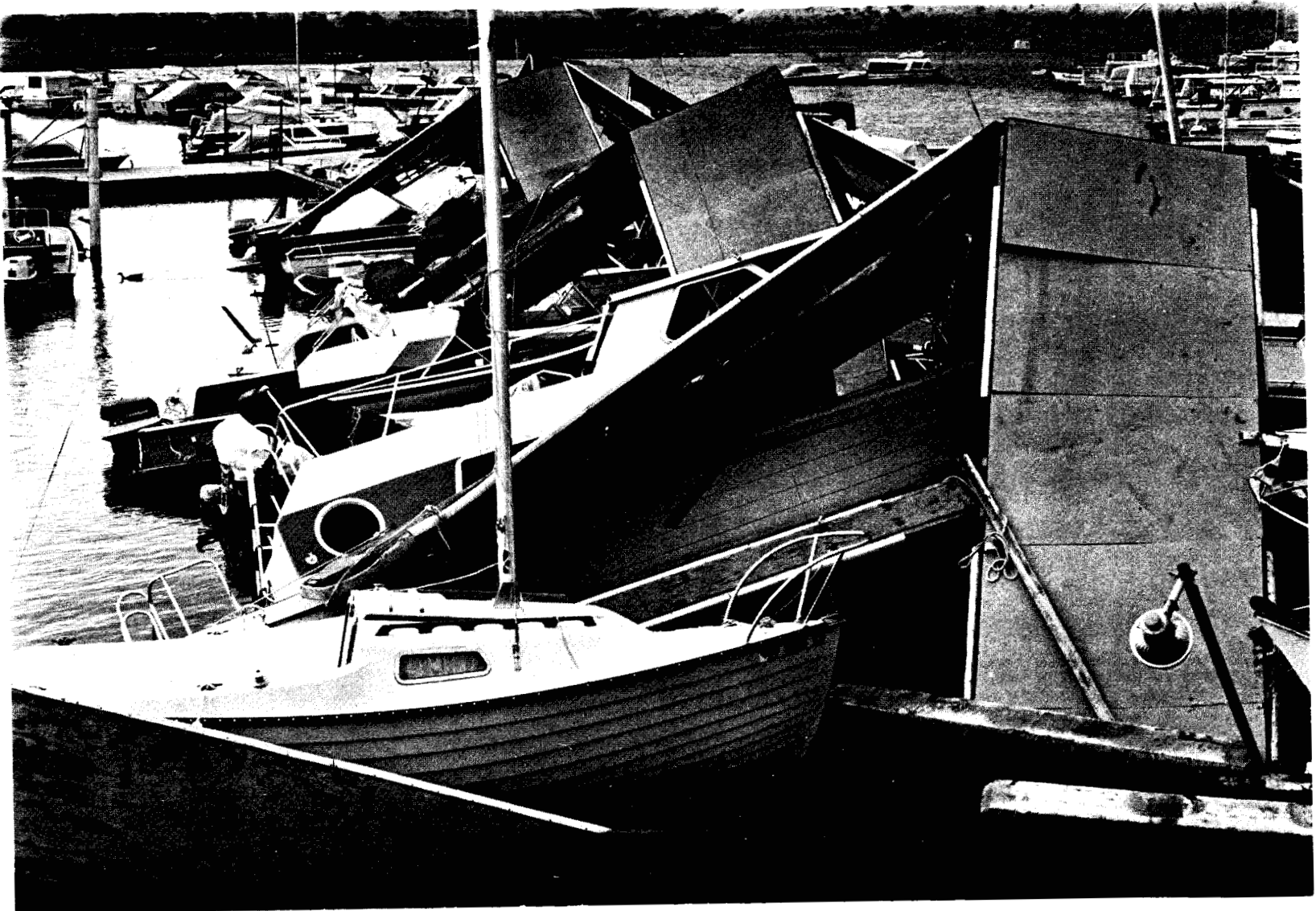
Figure 2. Lake Mead wind damages. (Photo: Bob McKeever)
