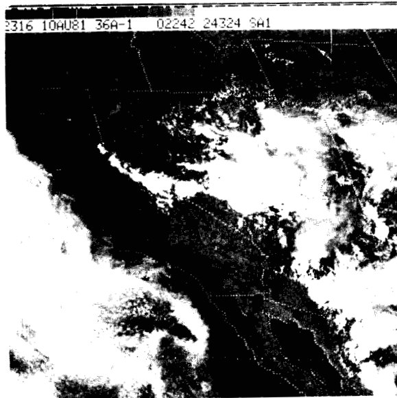
Figure 7. Infrared GOES Satellite imagery for 2316Z August 10, 1981.
