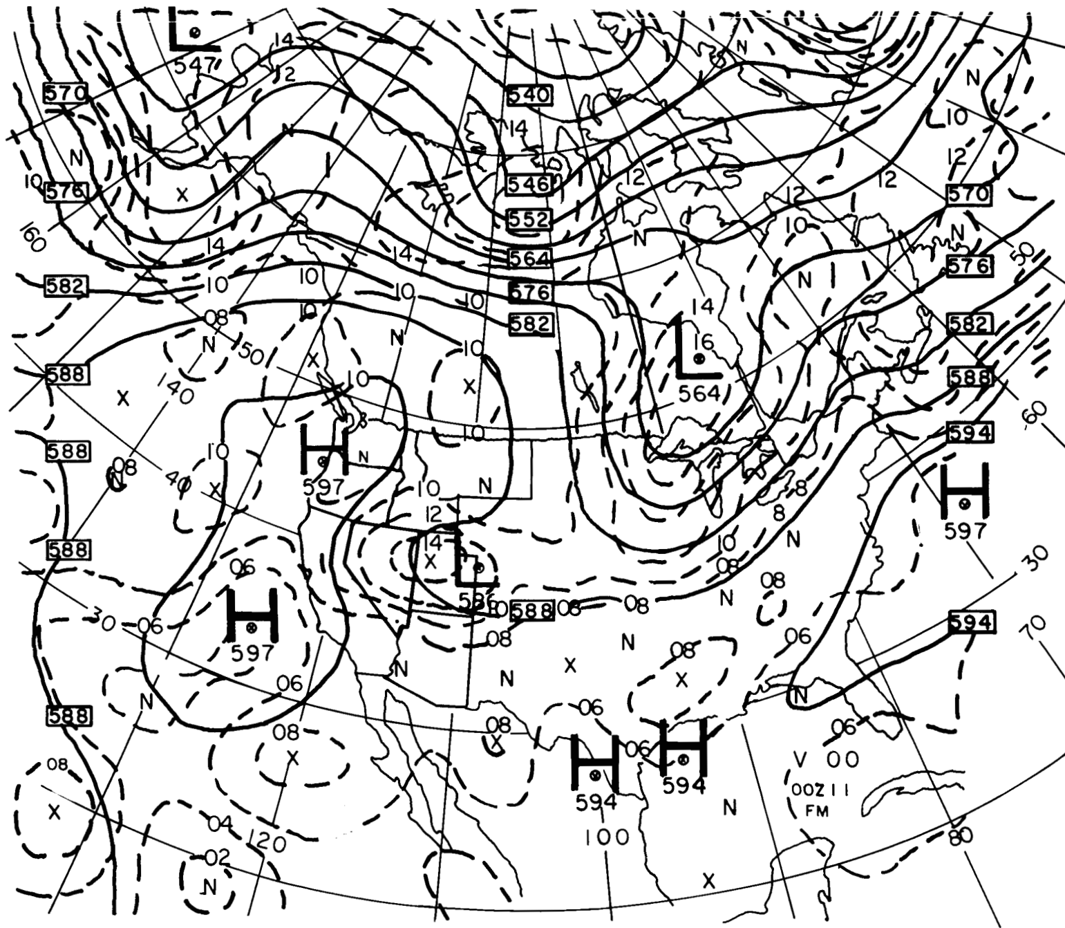
Figure 6. LFM 500 mb Analysis 00Z Tuesday, August 11, 1981
