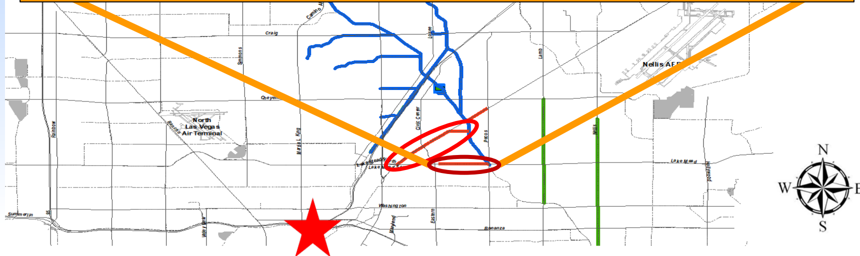
Lake Mead Storm Drain, Las Vegas Wash to Civic Center
