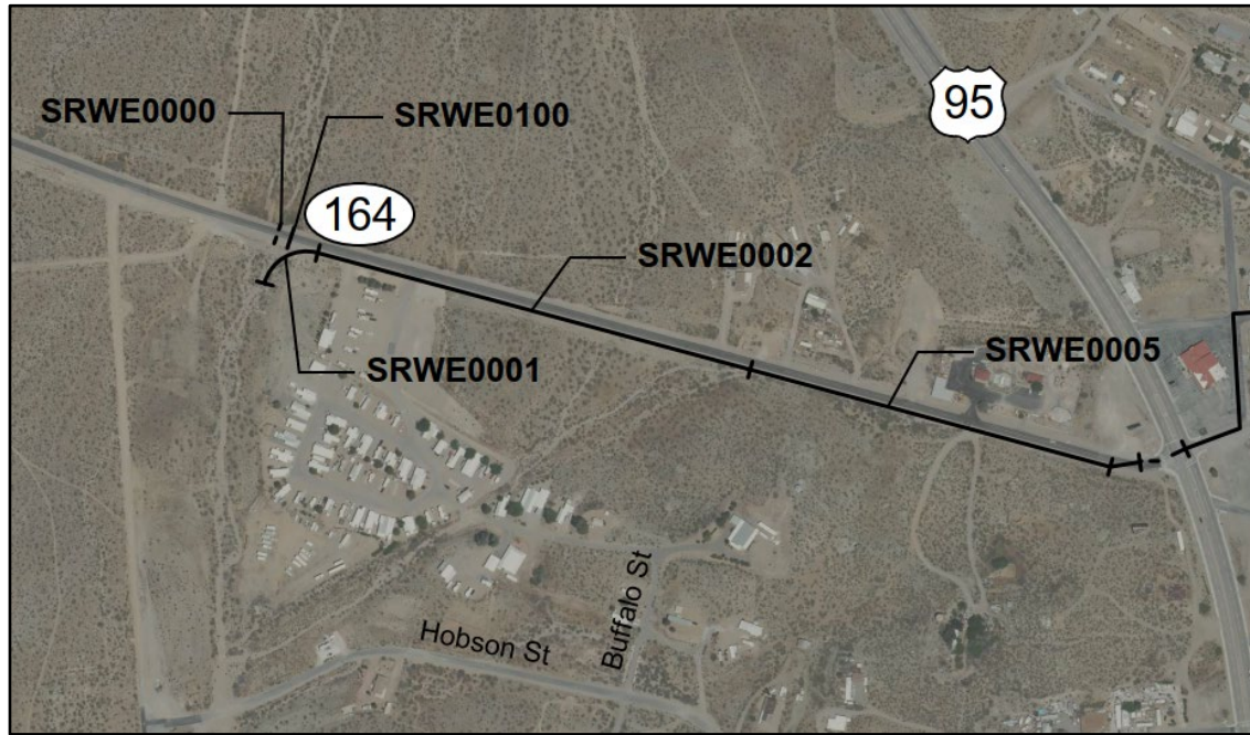
2019 OAMPU SEARCHLIGHT WEST FLOOD CONTROL FACILITIES
